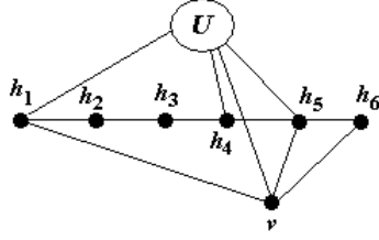
FIGURE 5: Lemma 8
