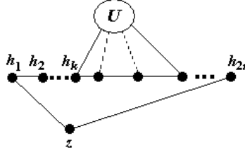
FIGURE 7: Lemma 10.1)
