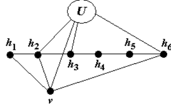
FIGURE 6: Lemma 9
