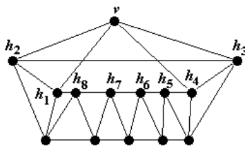
FIGURE 3: \alpha = r = 4
