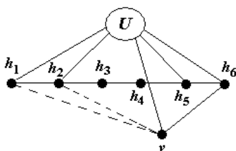
FIGURE 4: Lemma 7
