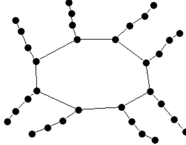
FIGURE 1: The 7-ciliate C(8, 3)
