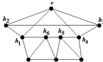
FIGURE 2: \alpha = r = 3
